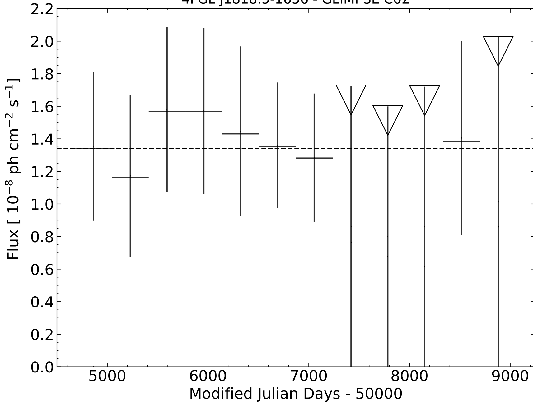
4FGL J1818.5-1656 - GLIMPSE C02
