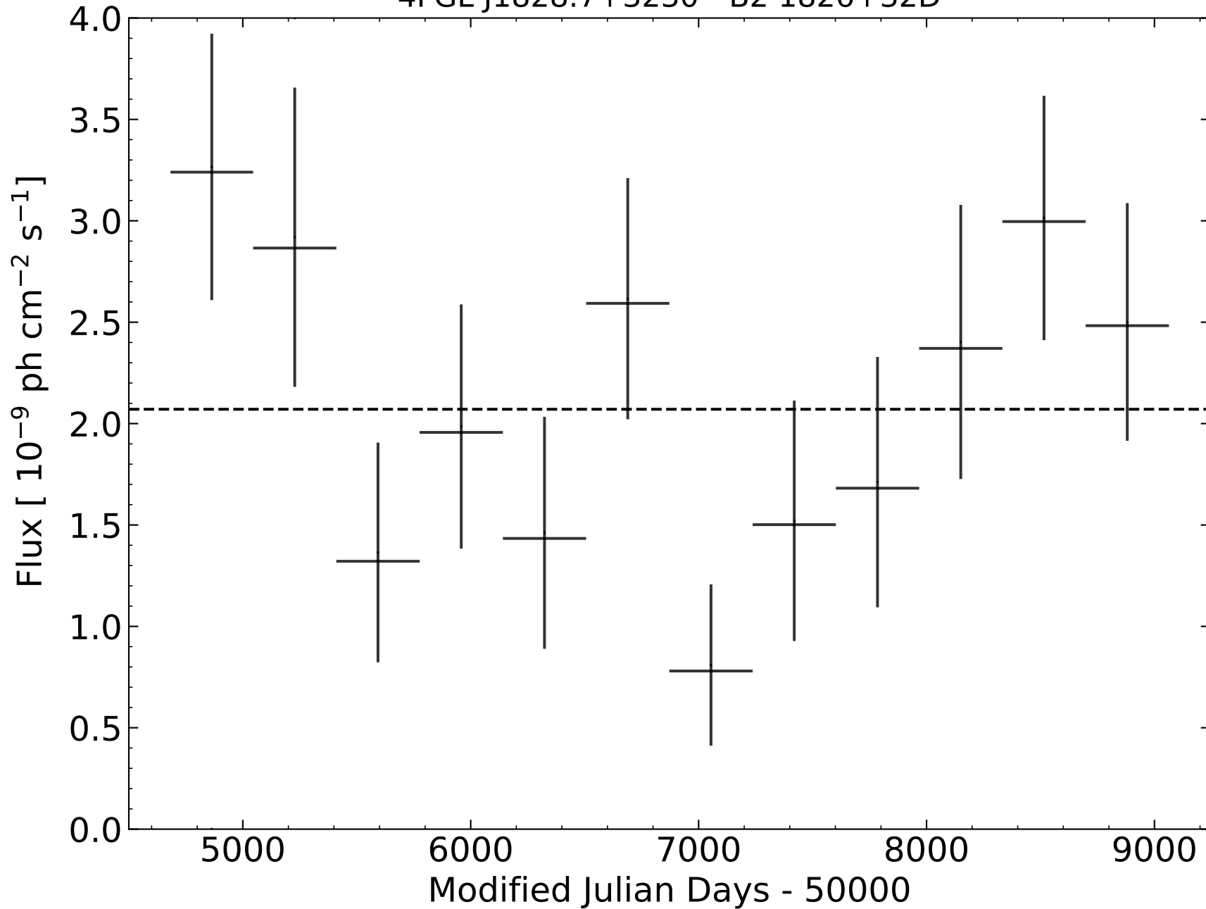
4FGL J1828.7+3230 - B2 1826+32D
