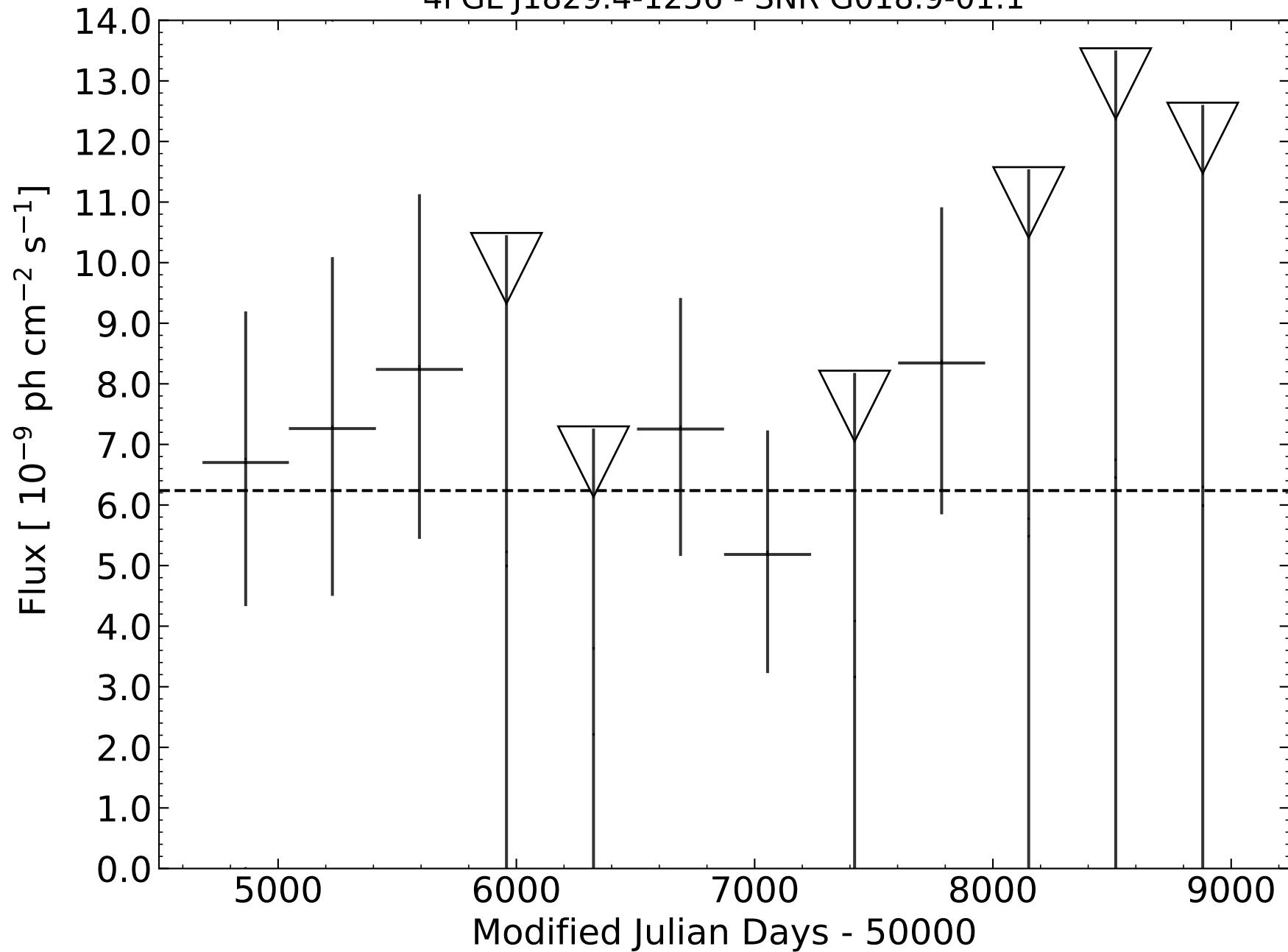
4FGL J1829.4-1256 - SNR G018.9-01.1
