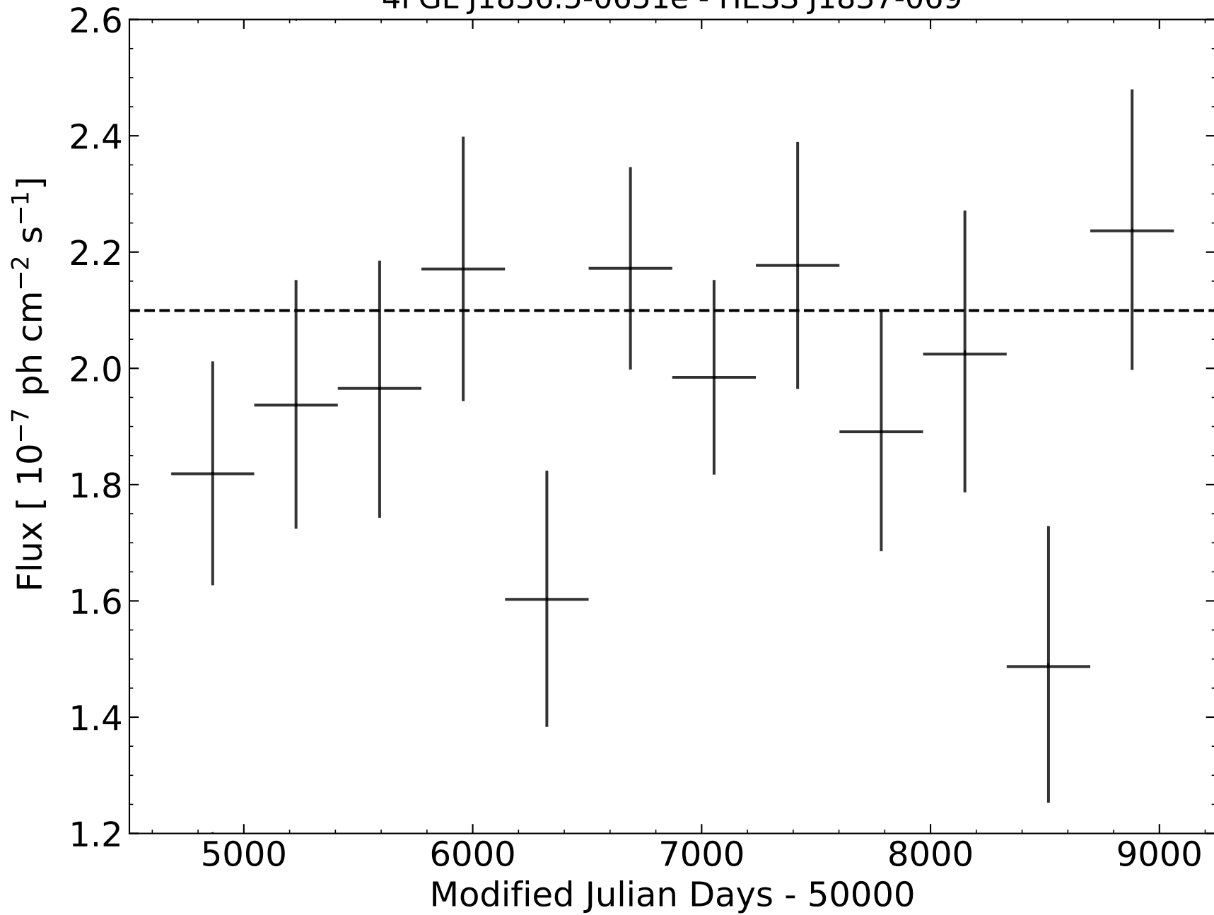
4FGL J1836.5-0651e - HESS J1837-069
