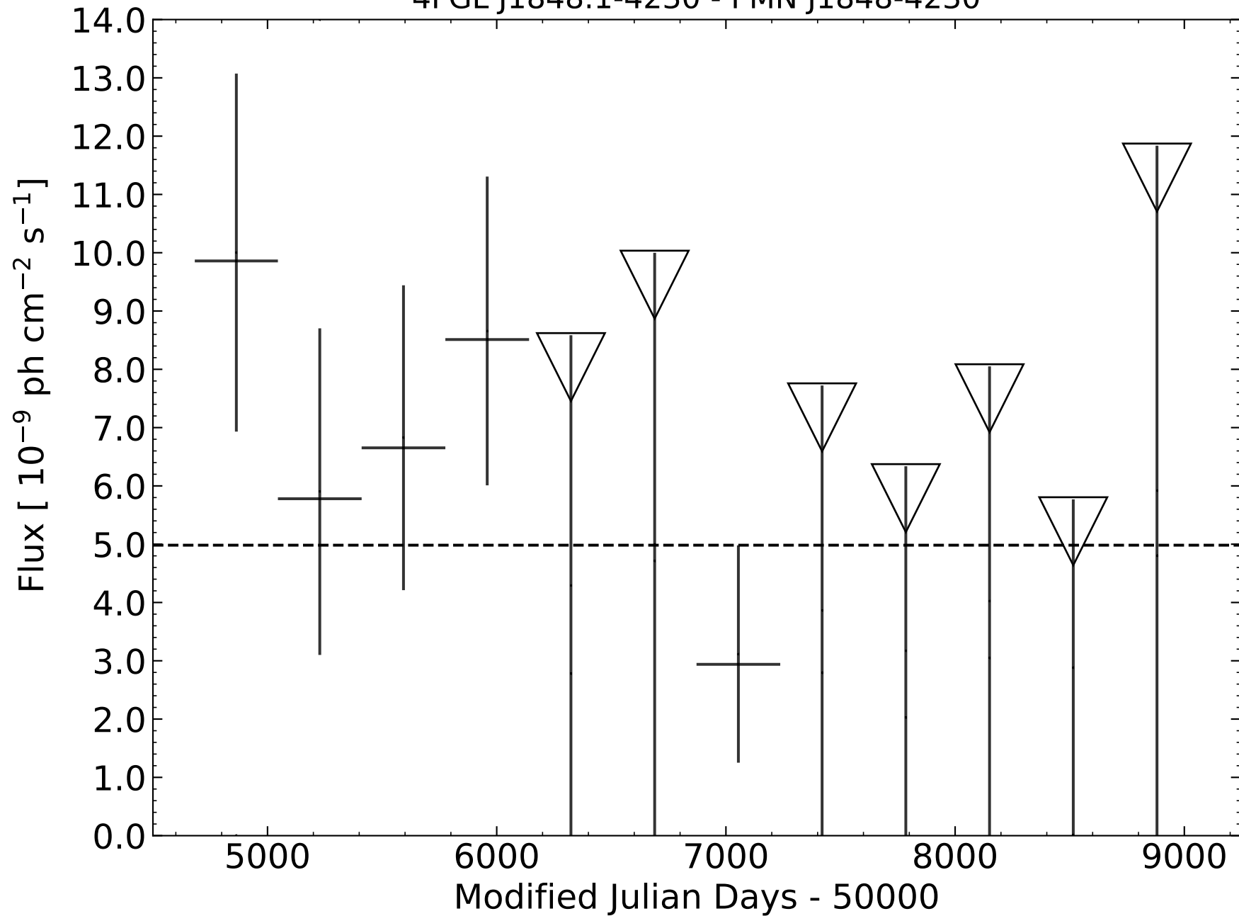
4FGL J1848.1-4230 - PMN J1848-4230
