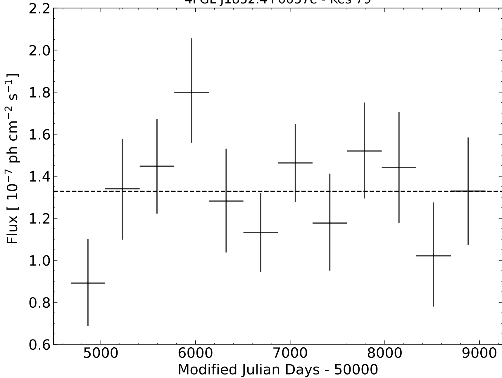
4FGL J1852.4+0037e - Kes 79
