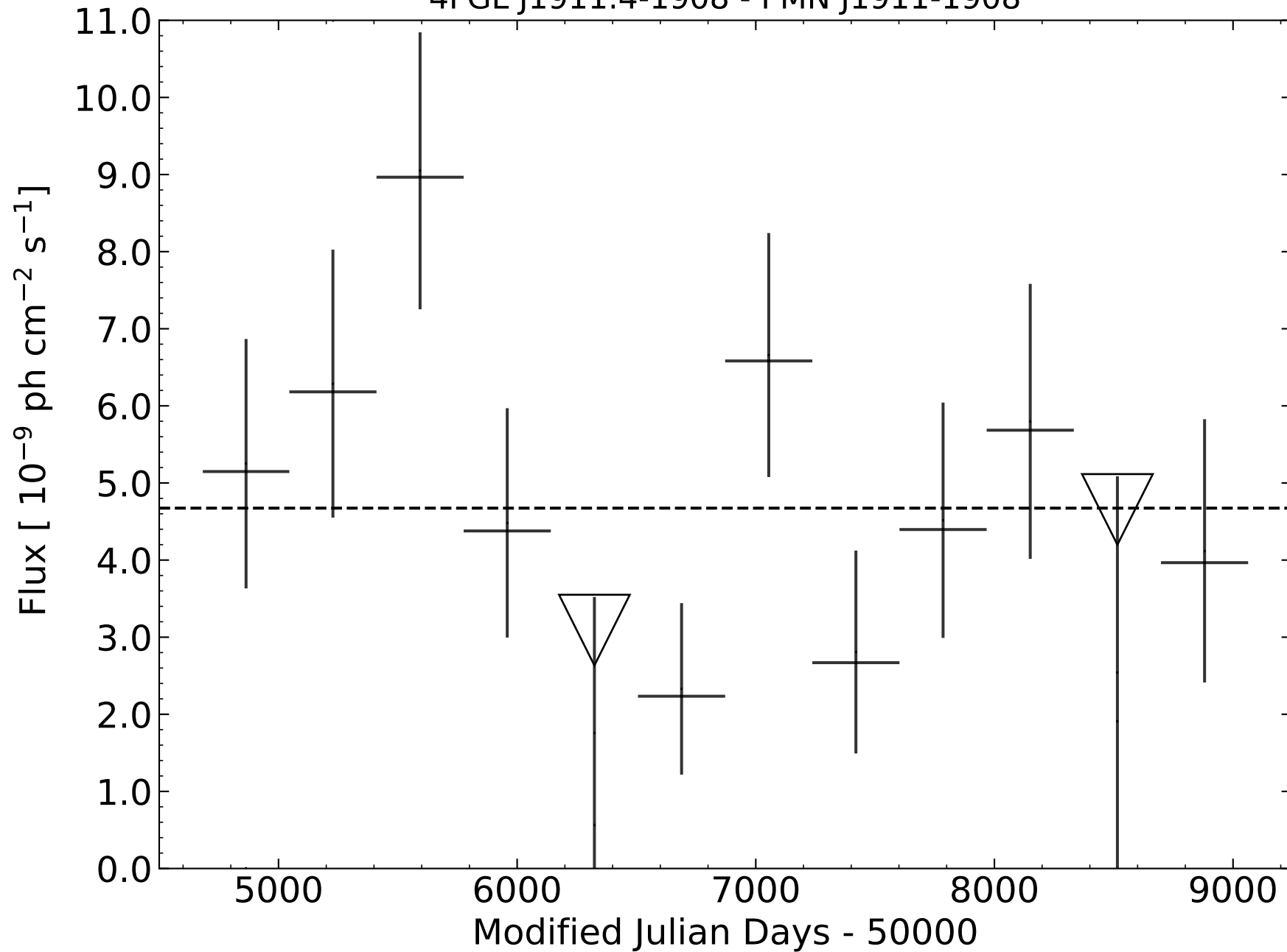
4FGL J1911.4-1908 - PMN J1911-1908
