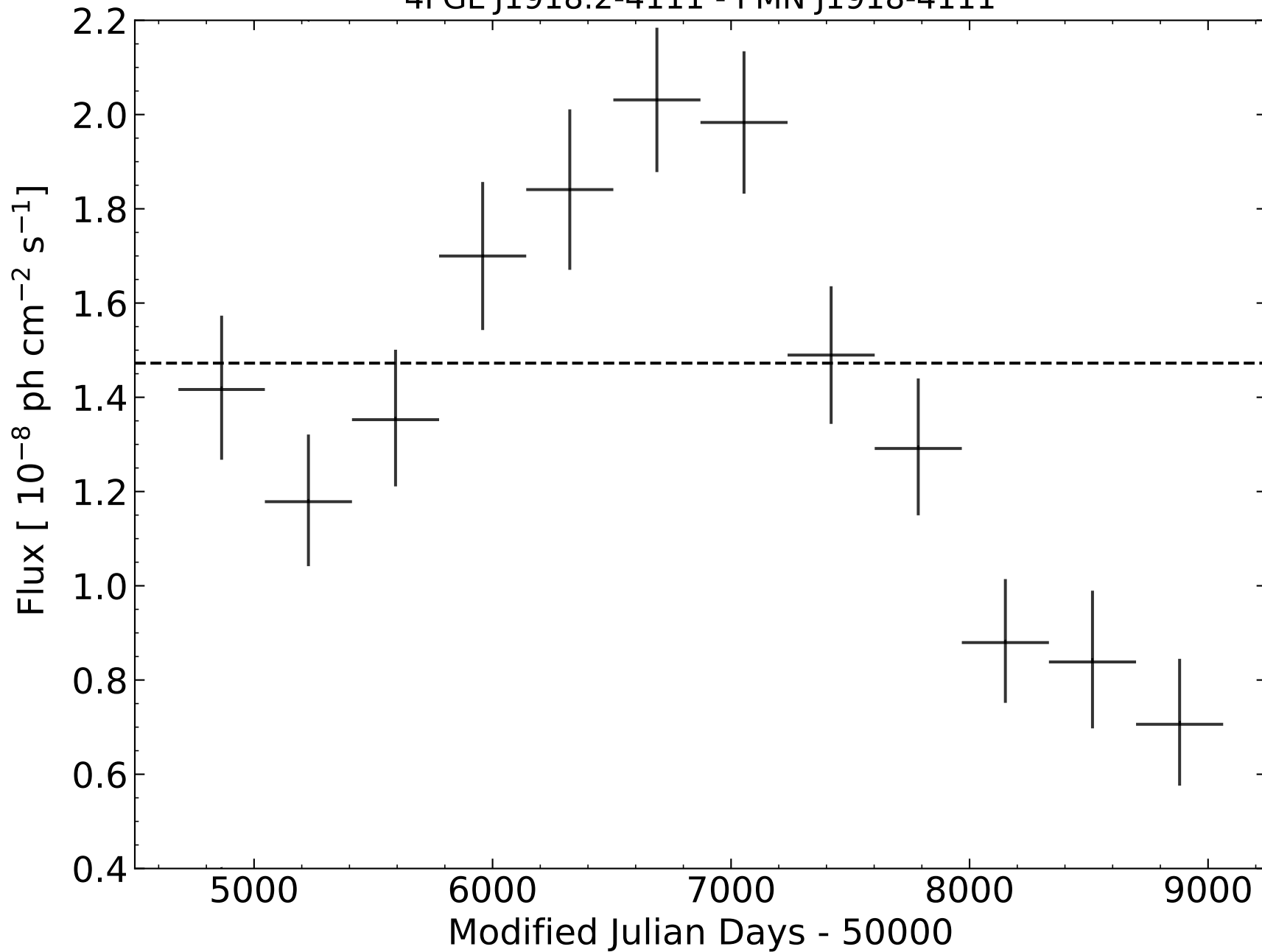
4FGL J1918.2-4111 - PMN J1918-4111
