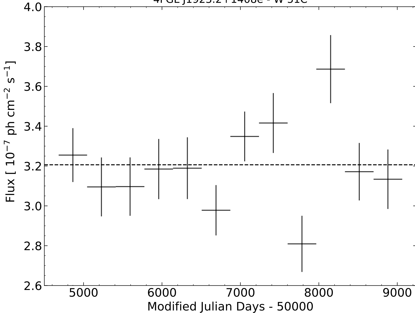
4FGL J1923.2+1408e - W 51C
