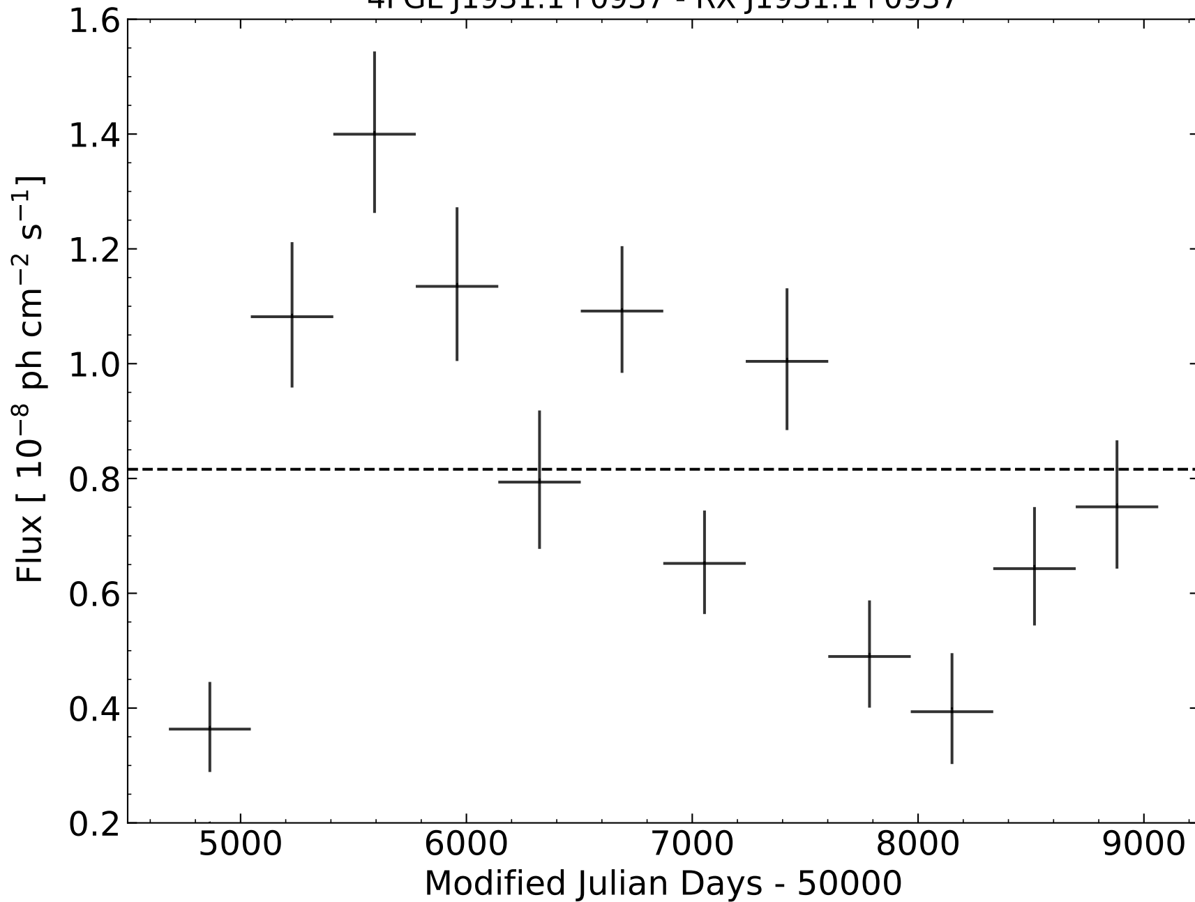
4FGL J1931.1+0937 - RX J1931.1+0937
