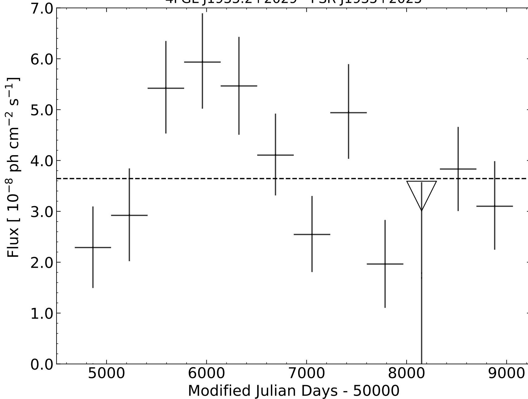
4FGL J1935.2+2029 - PSR J1935+2025
