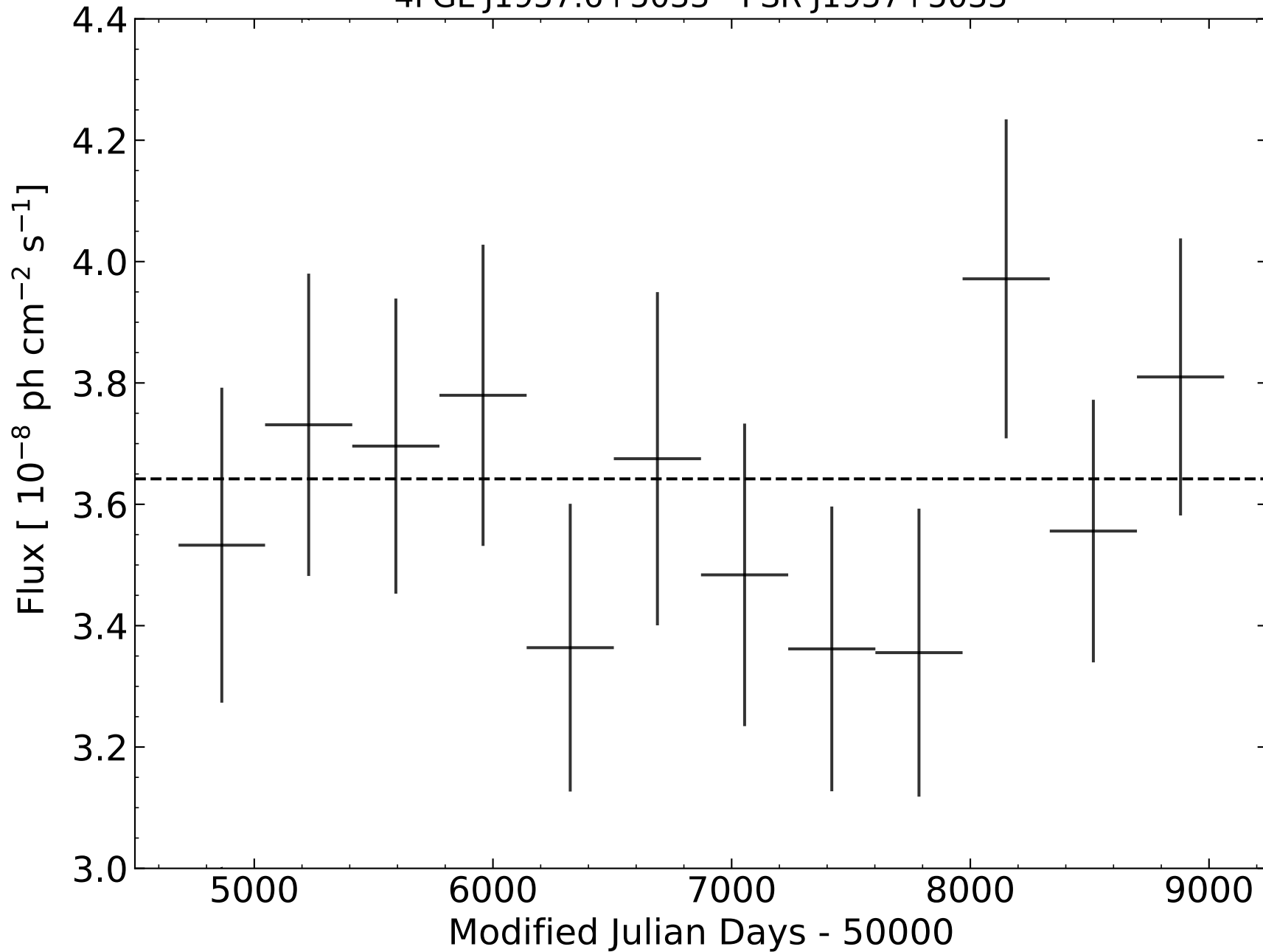
4FGL J1957.6+5033 - PSR J1957+5033
