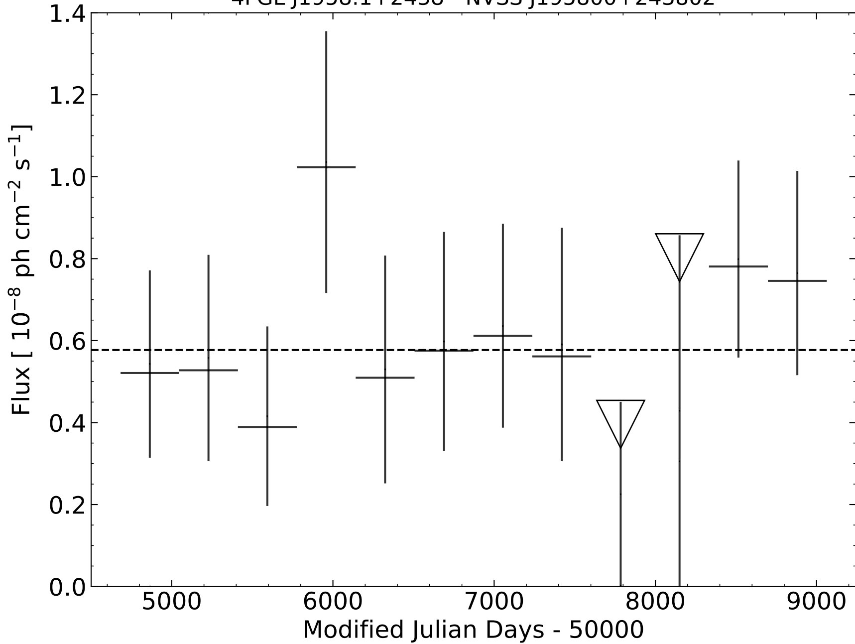
4FGL J1958.1+2438 - NVSS J195800+243802
