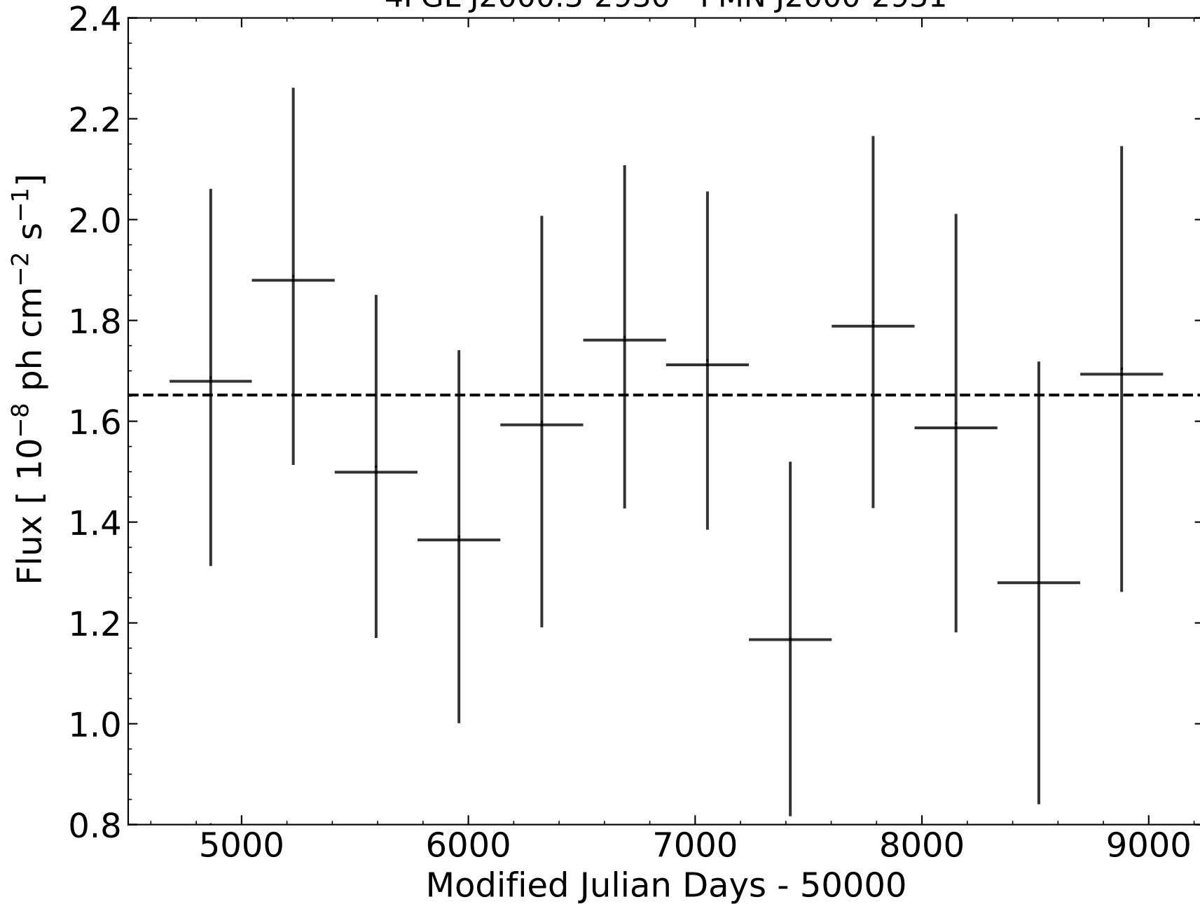
4FGL J2000.3-2930 - PMN J2000-2931
