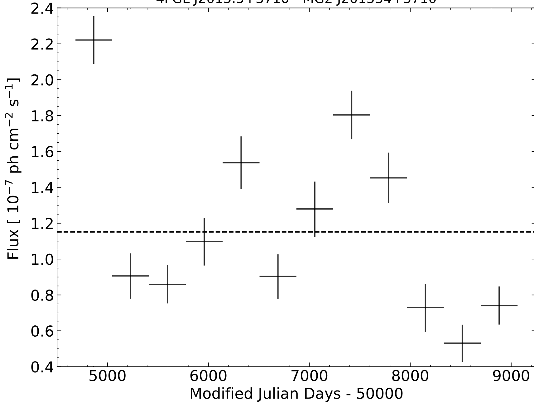
4FGL J2015.5+3710 - MG2 J201534+3710
