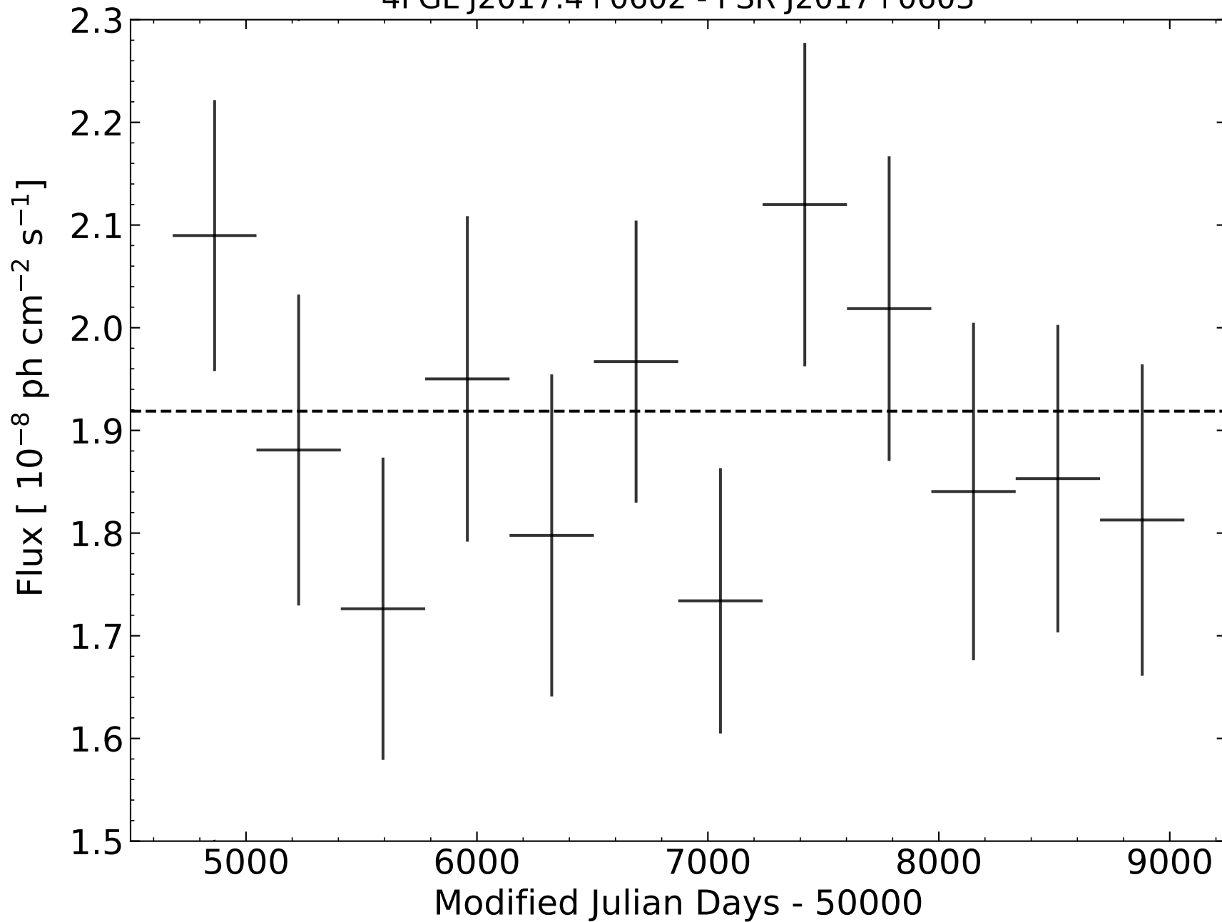
4FGL J2017.4+0602 - PSR J2017+0603
