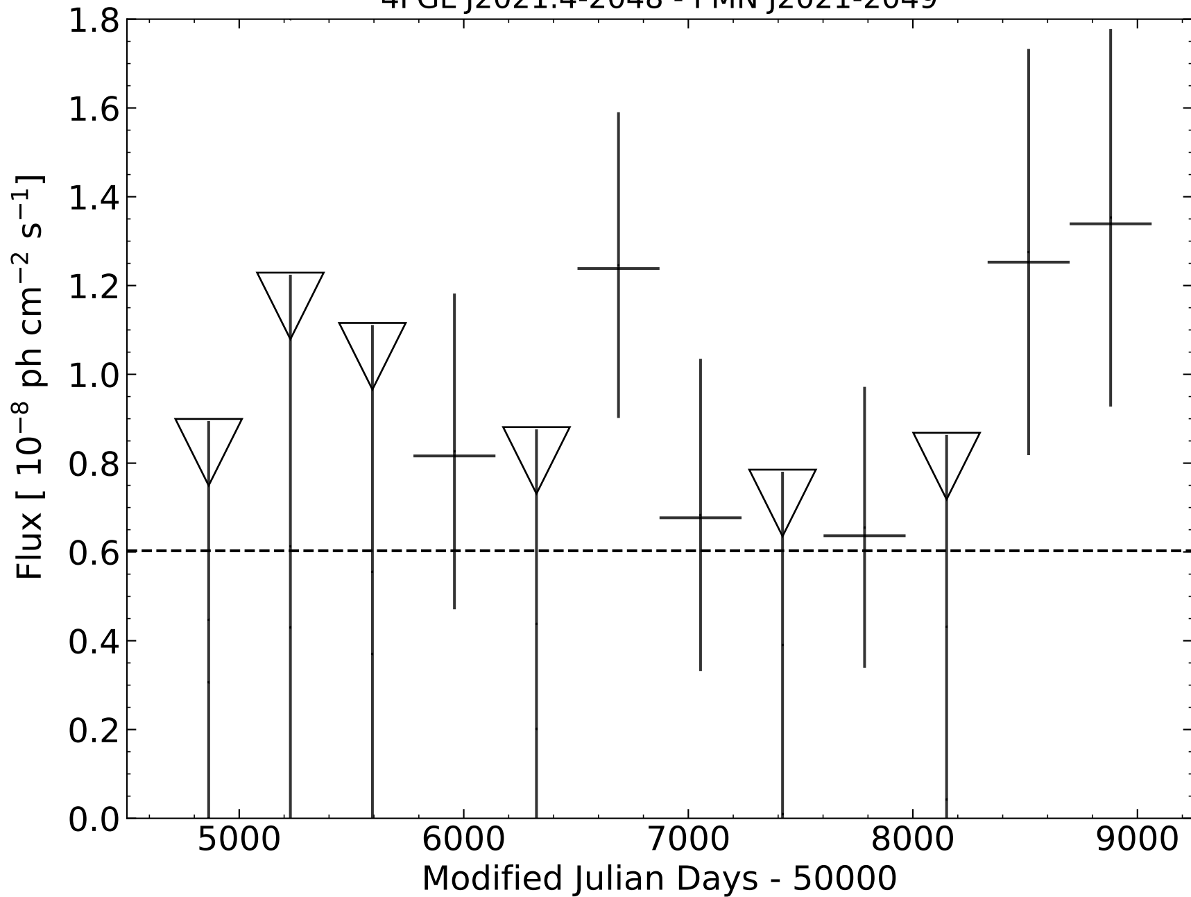
4FGL J2021.4-2048 - PMN J2021-2049
