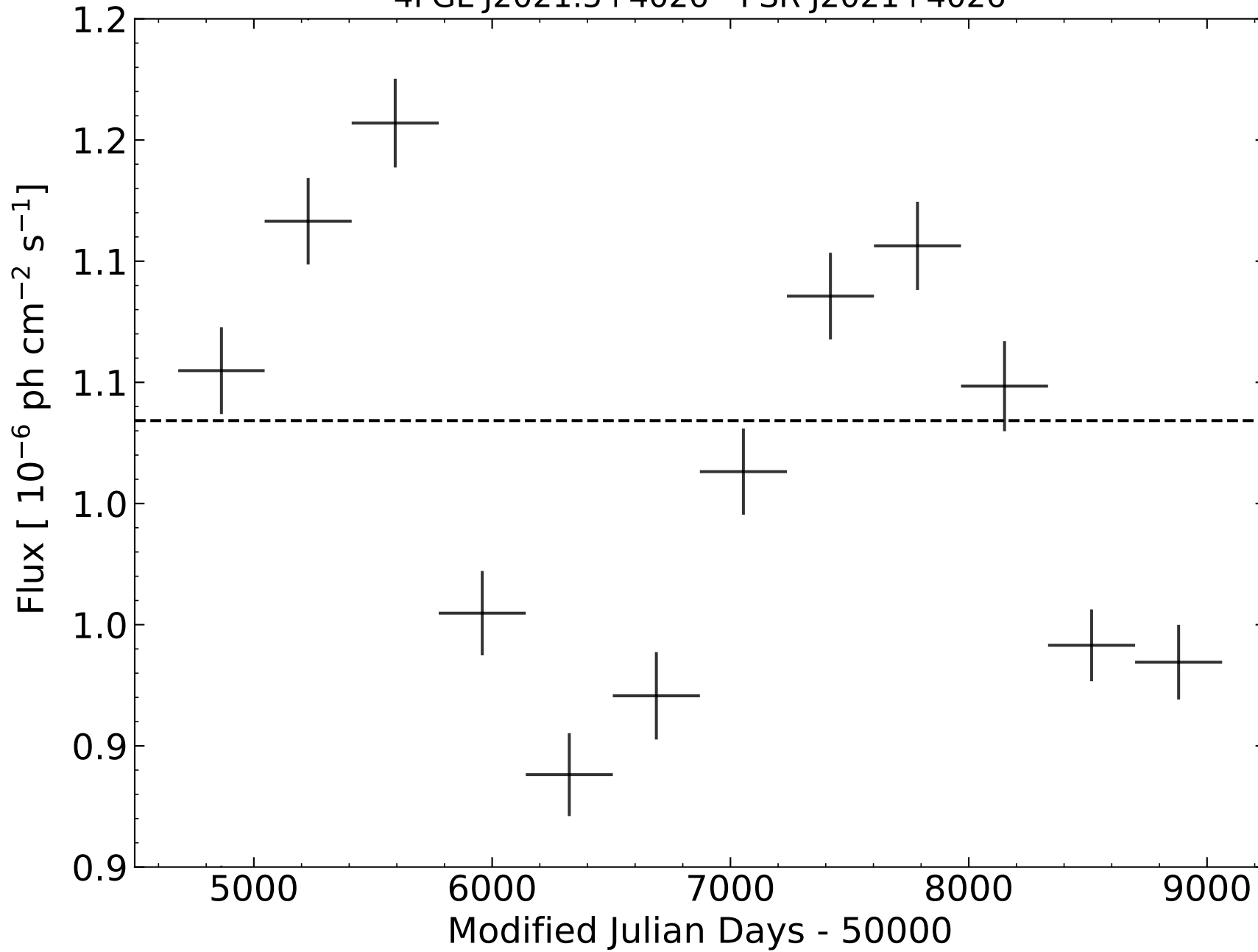
4FGL J2021.5+4026 - PSR J2021+4026
