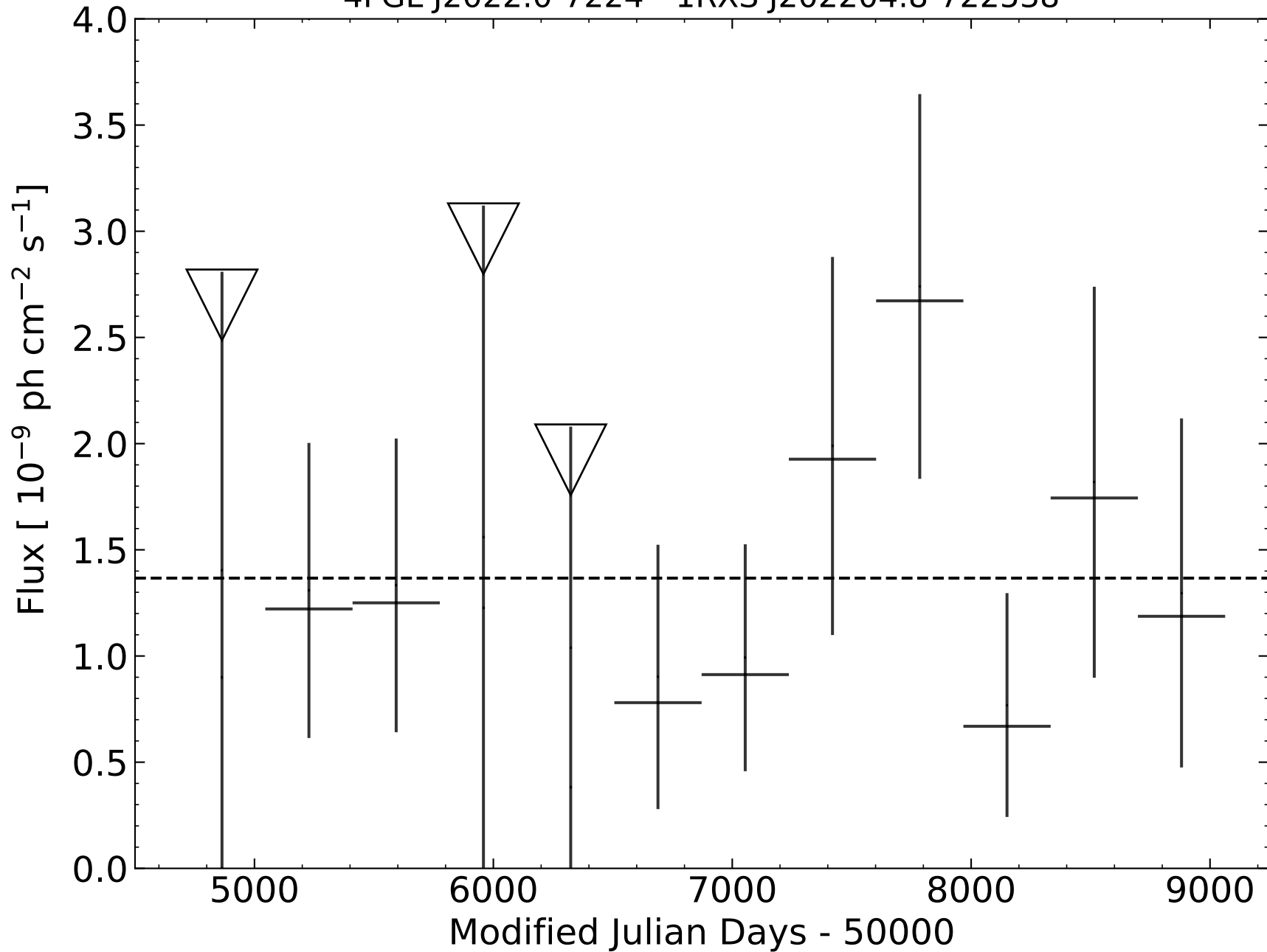
4FGL J2022.0-7224 - 1RXS J202204.8-722538
