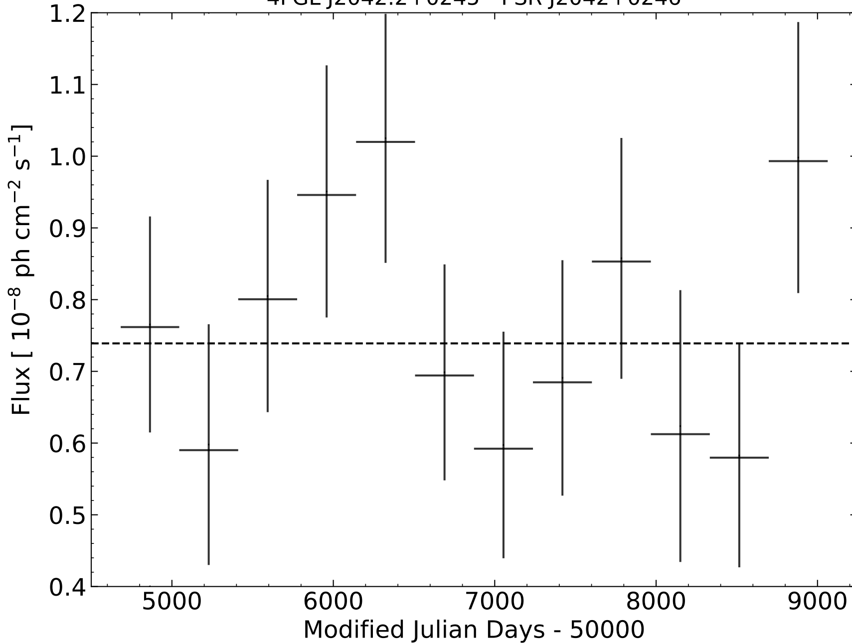
4FGL J2042.2+0245 - PSR J2042+0246
