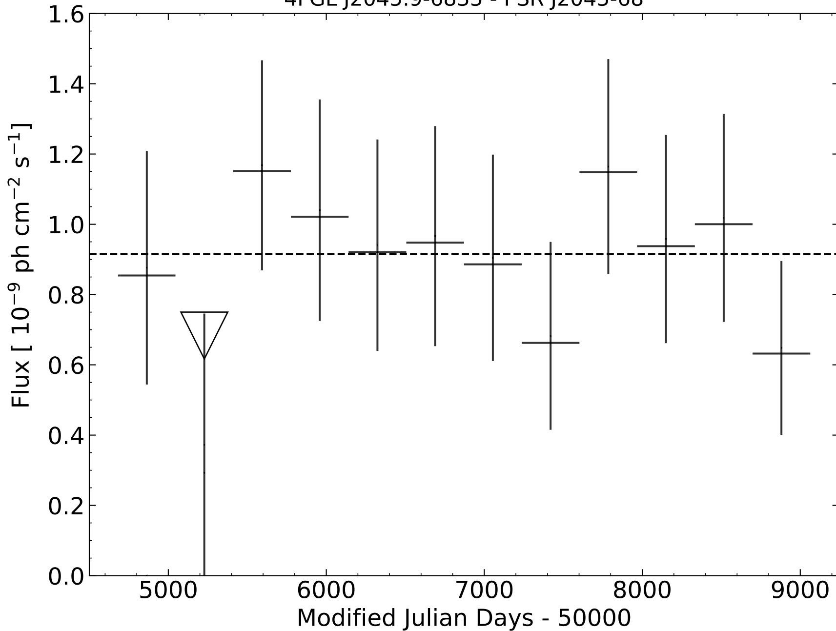
4FGL J2045.9-6835 - PSR J2045-68
