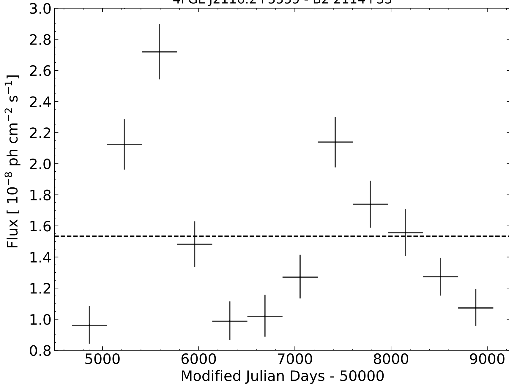
4FGL J2116.2+3339 - B2 2114+33
