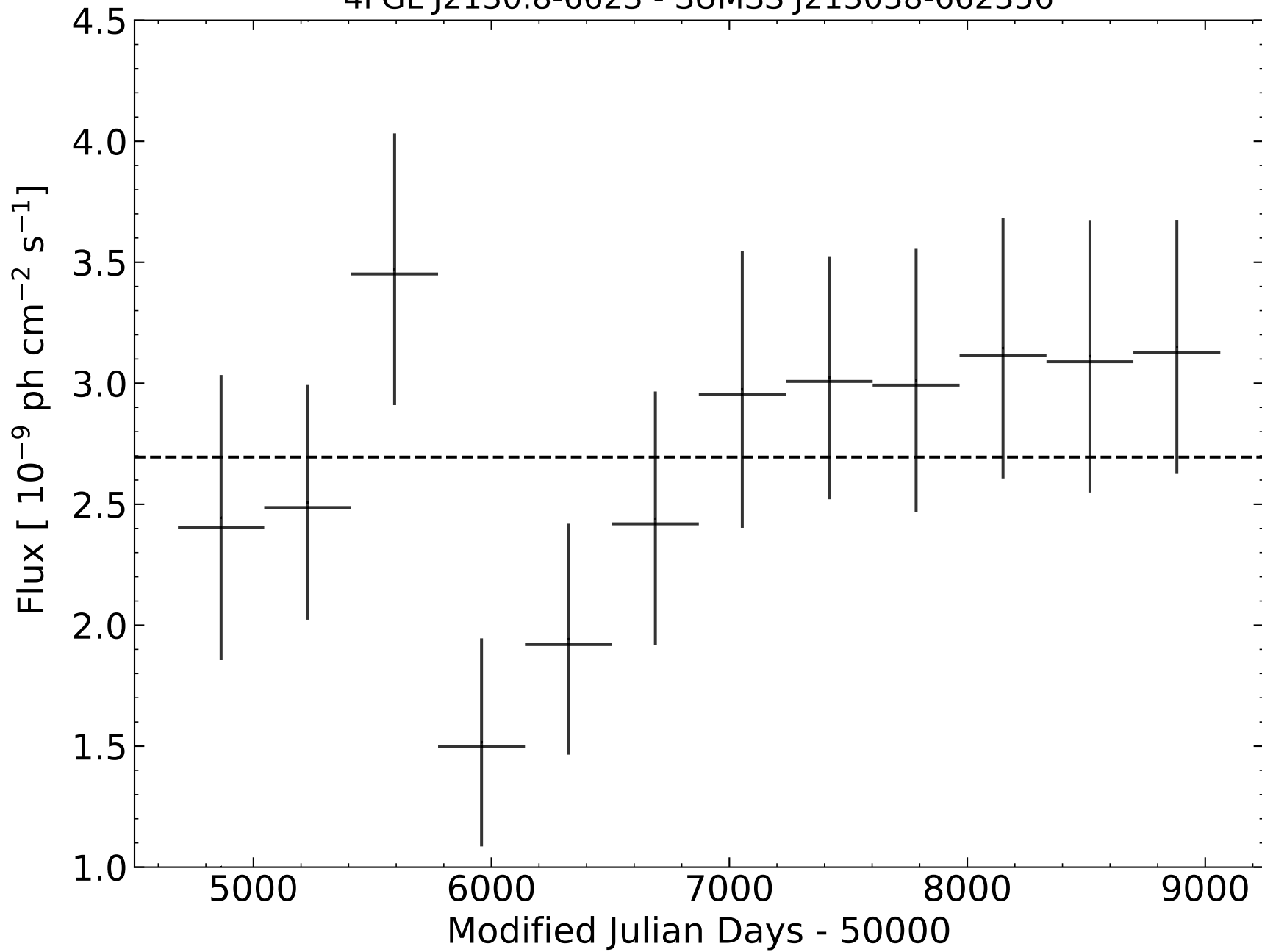
4FGL J2130.8-6623 - SUMSS J213038-662356
