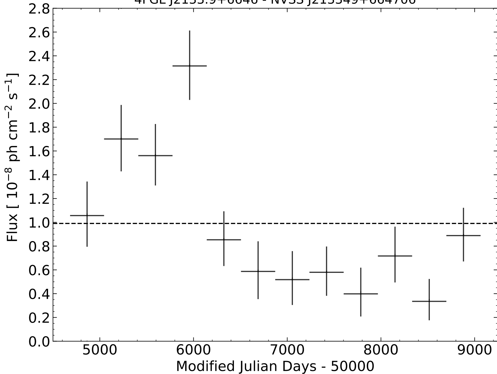
4FGL J2133.9+6646 - NVSS J213349+664706
