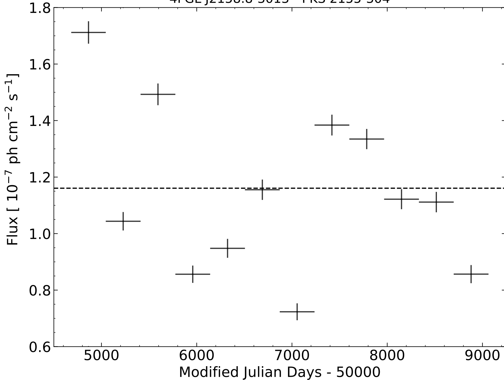
4FGL J2158.8-3013 - PKS 2155-304
