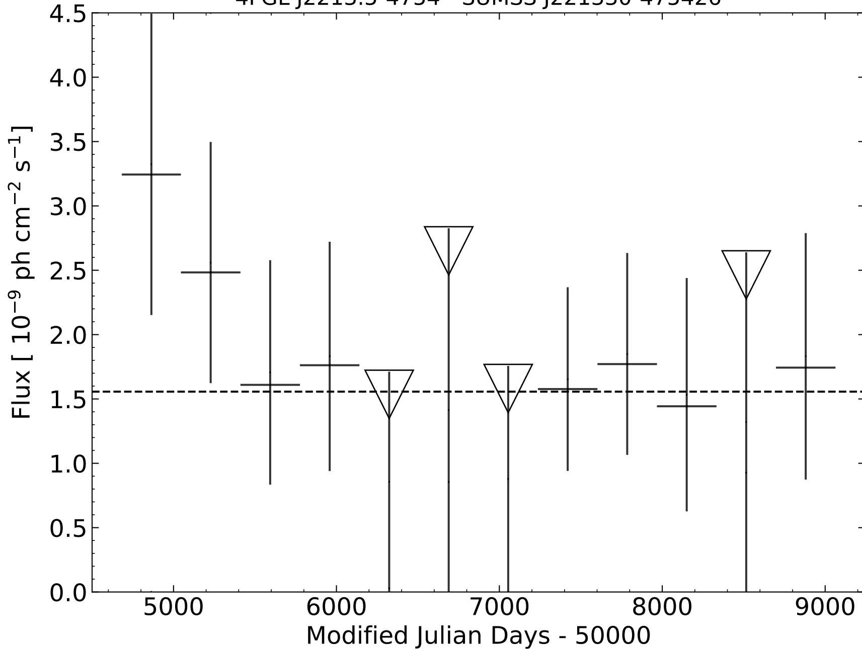
4FGL J2213.5-4754 - SUMSS J221330-475426
