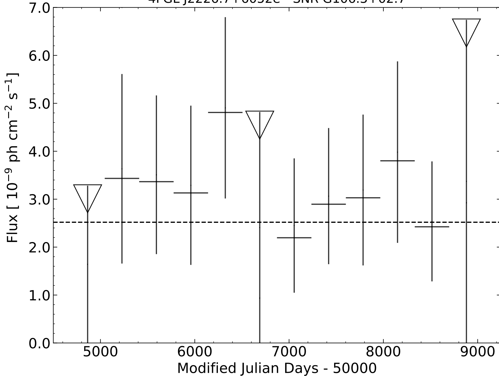
4FGL J2226.7+6052e - SNR G106.3+02.7
