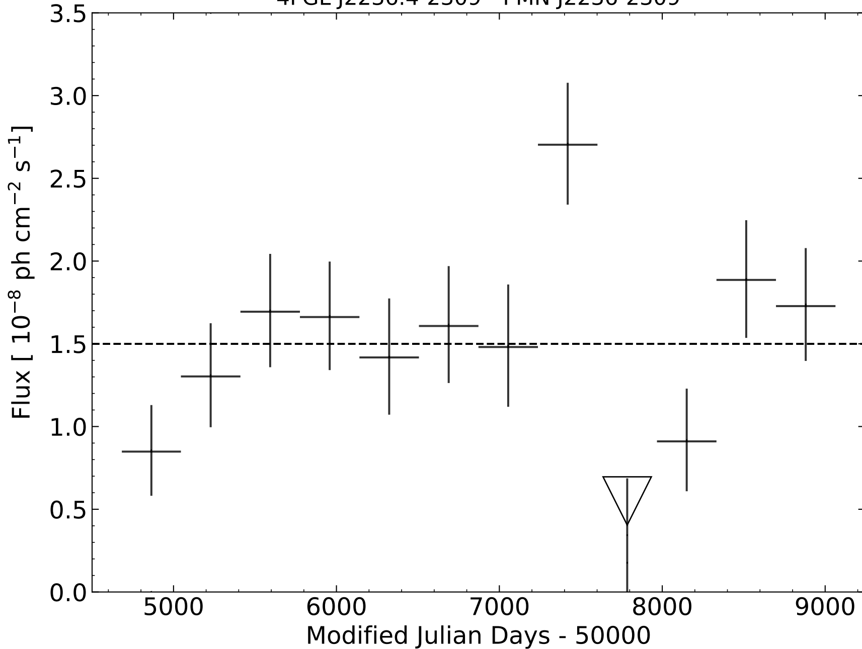
4FGL J2236.4-2309 - PMN J2236-2309
