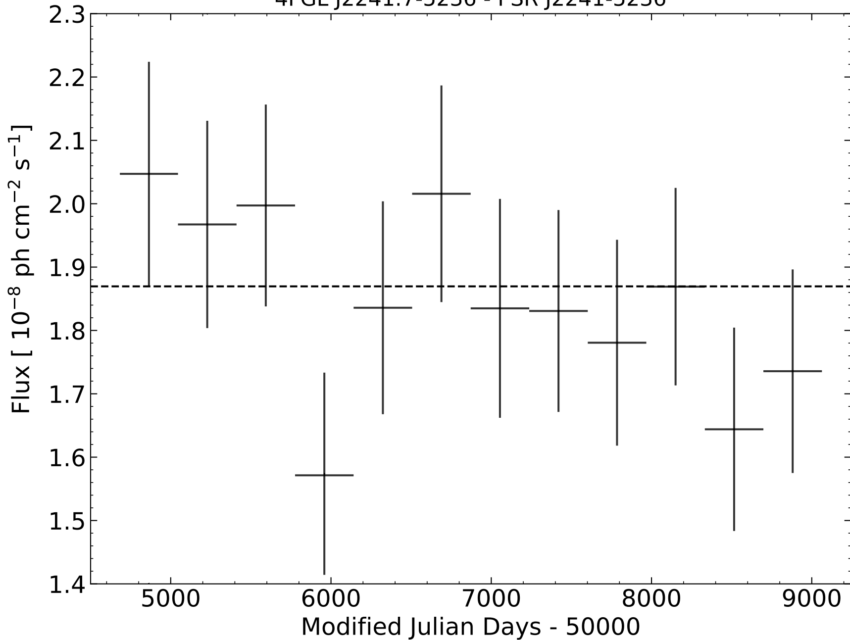
4FGL J2241.7-5236 - PSR J2241-5236
