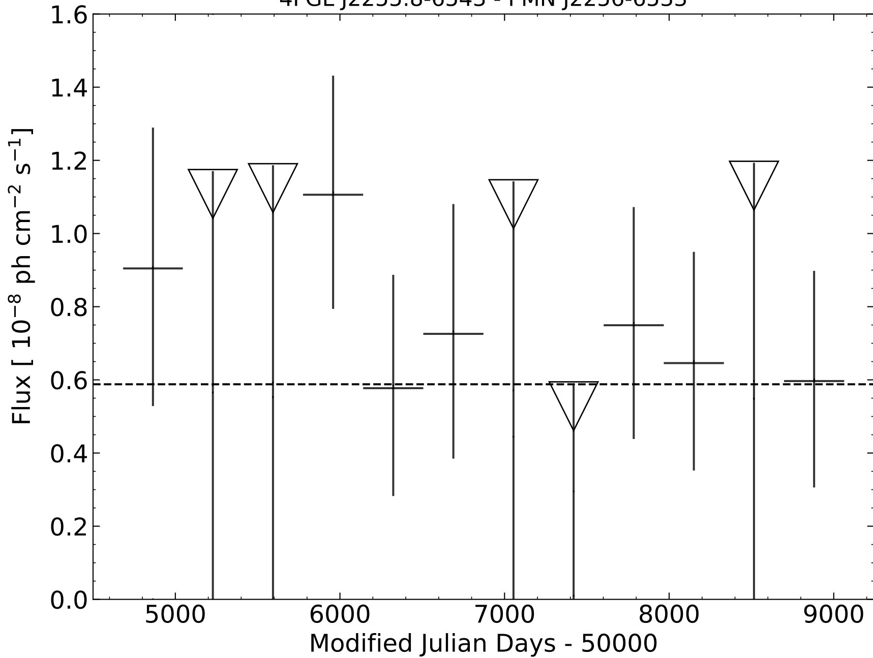
4FGL J2255.8-6543 - PMN J2256-6533
