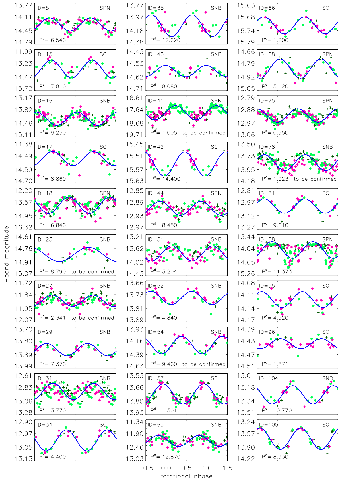
Figure 11. I-band light curves of our periodic variables vs. rotation phase. Phases are computed using the rotation period reported in Table 5. Different symbols are used to distinguish data belonging to different time intervals. The solid line represents the sinusoidal fit to the data.
