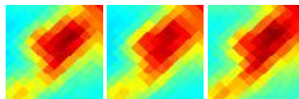
G168.85-15.83 J0417+281
