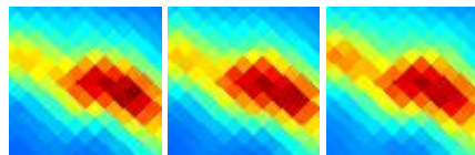
G170.81-18.34 J0415+250
