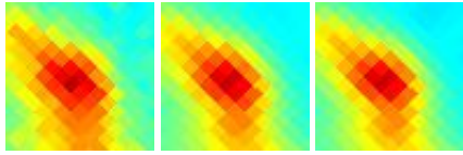
G120.98+02.66 J0032+654
