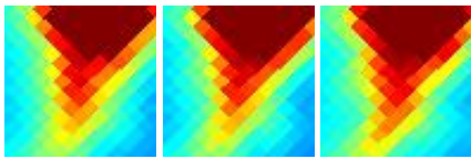
G158.86-21.60 J0327+301
