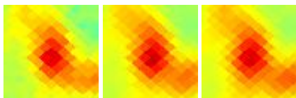
G159.58-32.84 J0301+206
