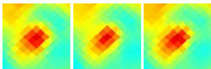
G174.06-15.81 J0432+243
