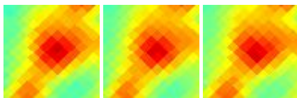
G005.31+10.78 J1718-186
