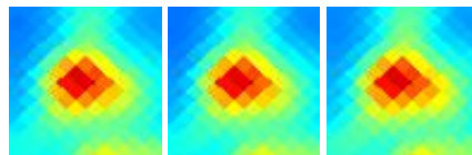
G103.49+13.07 J2106+670
