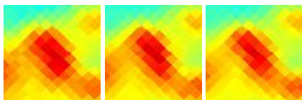
G005.29+14.47 J1705-166
