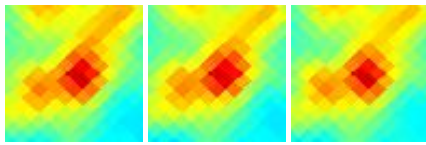
G338.13+16.37 J1540-346
