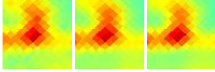
G139.17+15.07 J0430+706
