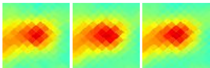
G170.00-16.14 J0420+270
