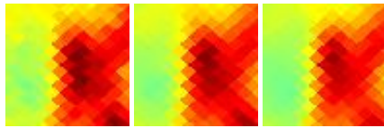
G121.92-01.71 J0043+611
