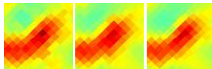
G174.81-15.15 J0437+242
