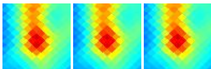
G303.15-16.33 J1256-792
