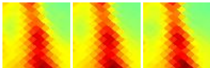
G060.75-01.23 J1950+239
