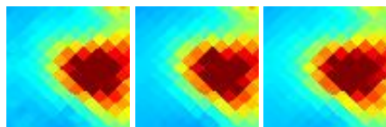
G172.15-16.02 J0426+256
