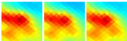
G151.08+04.46 J0430+548
