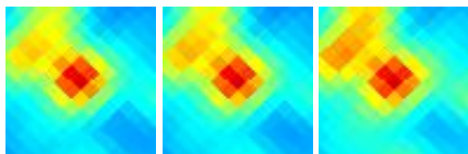
G111.77+13.78 J2210+730
