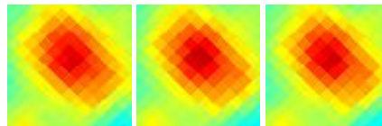
G182.02-00.16 J0549+271
