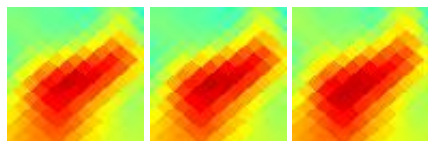
G093.91+10.02 J2037+577
