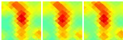
G337.58+16.35 J1538-350
