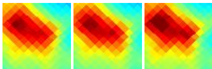
G159.67-34.31 J0257+193
