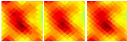
G144.44+08.55 J0417+624
