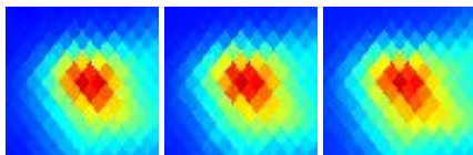
G006.41+20.56 J1647-122
