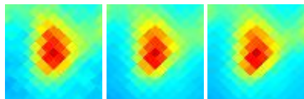
G172.85-14.74 J0433+259
