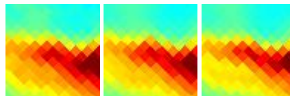
G007.80+21.10 J1648-108
