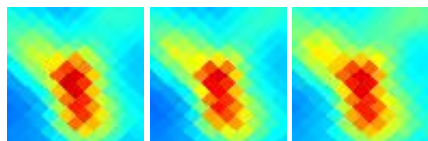
G171.91-15.65 J0427+260
