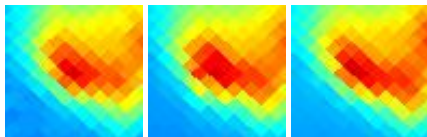
G004.15+35.77 J1553-046
