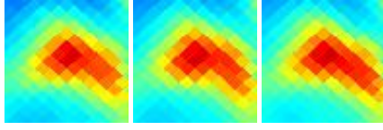
G338.88+09.48 J1605-394
