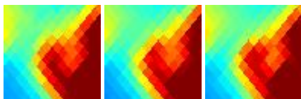
G159.65-19.68 J0336+312
