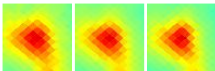
G147.96-08.02 J0324+472
