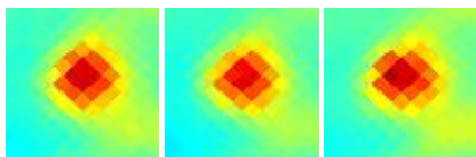
G214.43-19.90 J0542-102
