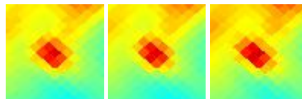
G026.93-20.68 J1956-143
