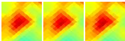
G129.90+11.62 J0228+731
