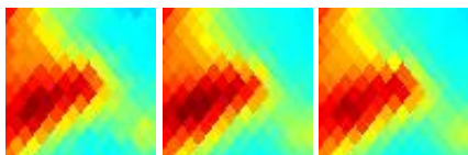
G004.92+17.95 J1652-148
