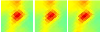
G140.77+05.00 J0334+620
