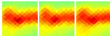
G176.17-02.10 J0527+310
