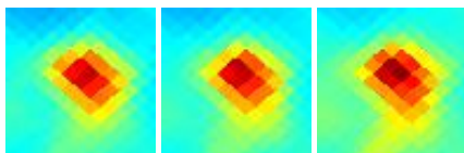
G162.83-18.44 J0350+302
