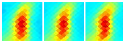
G224.47-00.65 J0710-105
