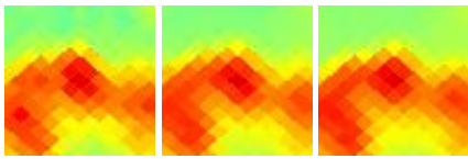
G159.16-05.58 J0421+420
