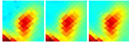
G338.79+17.23 J1540-336
