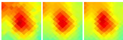
G163.21-08.40 J0425+372
