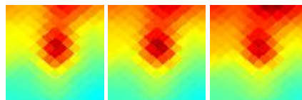
G047.74-05.56 J1938+105
