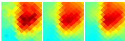
G103.77+13.90 J2102+677
