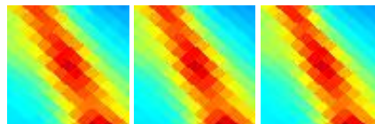
G301.20-16.54 J1215-792
