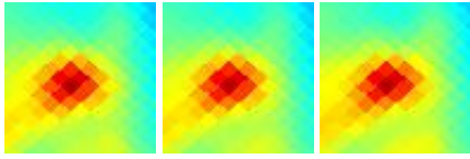
G133.72-45.31 J0123+168
