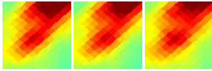
G343.89-02.42 J1711-436
