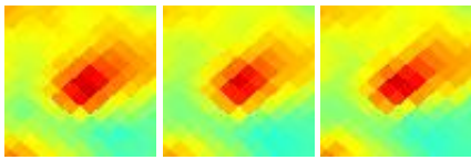
G156.42+32.53 J0806+605
