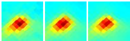
G004.02+16.64 J1655-163
