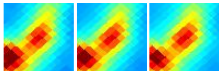
G049.06-04.18 J1936+123
