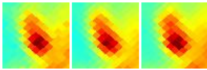
G156.53-08.63 J0359+416
