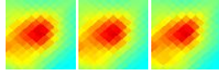
G238.71-01.47 J0735-234
