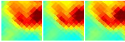
G338.68+11.85 J1556-378
