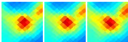
G049.76-07.25 J1948+114
