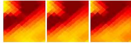
G237.30-04.76 J0719-238
