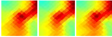
G358.79+05.64 J1721-268
