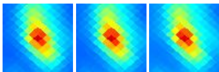
G320.66-03.67 J1527-610
