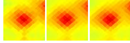
G248.97-03.20 J0751-332
