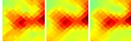
G140.49+06.07 J0337+631
