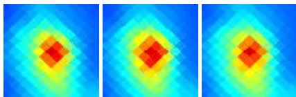
G174.88-17.11 J0430+229
