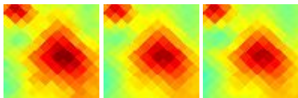
G222.95-05.45 J0650-113
