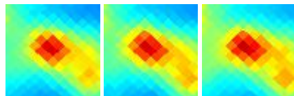
G171.32+04.40 J0541+386
