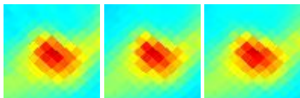
G023.37+08.21 J1804-046
