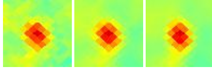
G255.43-03.95 J0805-391
