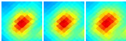
G336.95+09.17 J1559-409
