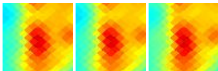
G266.96-04.64 J0838-490
