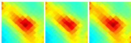
G174.70-15.48 J0435+241
