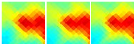
G154.95-15.19 J0332+374
