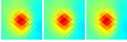
G089.64-06.59 J2137+433
