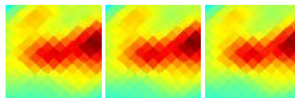
G300.60-03.13 J1228-659
