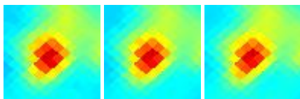
G131.72+09.70 J0239+707
