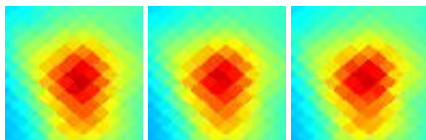
G153.34+11.26 J0519+573
