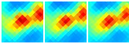
G158.88-34.18 J0255+198
