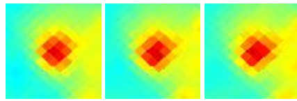
G156.90-08.49 J0401+414
