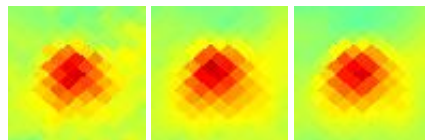
G175.31-20.50 J0420+204
