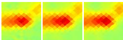
G300.69-09.40 J1222-721
