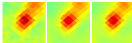
G335.63+08.12 J1557-426
