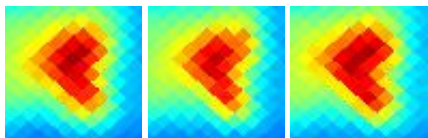
G003.27+10.42 J1714-205
