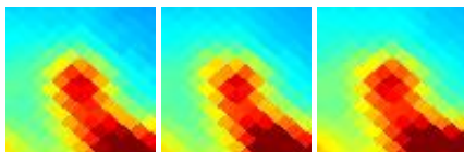
G181.71+04.16 J0606+295
