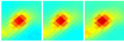
G350.35+04.40 J1702-344
