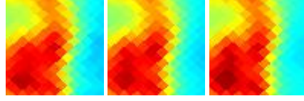
G089.93-07.03 J2139+432
