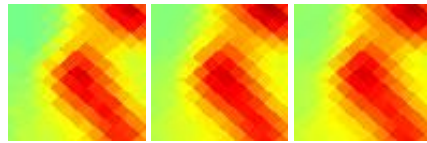
G144.49+08.70 J0419+625
