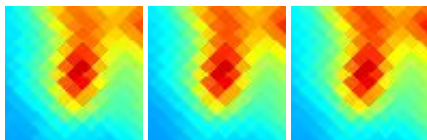
G111.97+20.52 J2055+780
