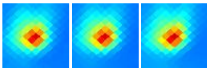
G110.96+19.49 J2100+766
