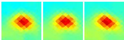
G335.89-02.64 J1643-500
