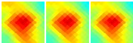
G108.10+13.19 J2140+703
