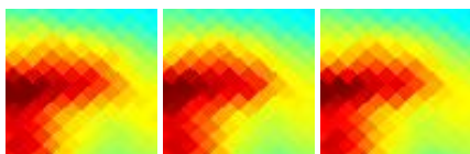
G173.36-16.27 J0429+246
