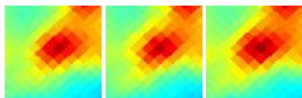
G172.94-05.49 J0506+317
