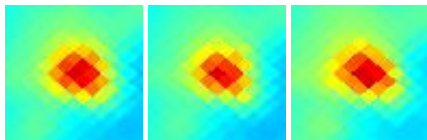
G031.44+04.18 J1833+005
