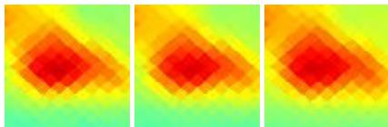
G098.06+13.97 J2029+633
