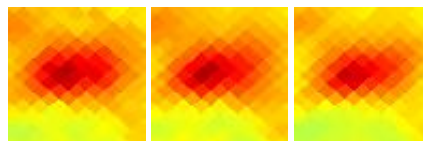
G163.32-08.42 J0425+371
