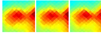
G359.71-18.20 J1903-372
