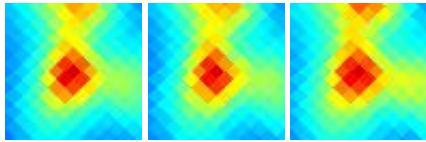
G359.78-18.34 J1903-372
