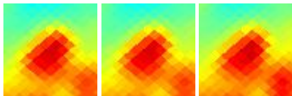
G269.67+05.41 J0932-442
