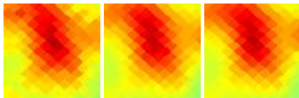
G154.07+05.21 J0447+531
