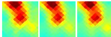
G217.79-17.36 J0557-120
