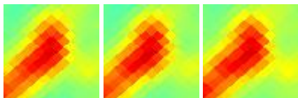
G027.09-20.70 J1956-142
