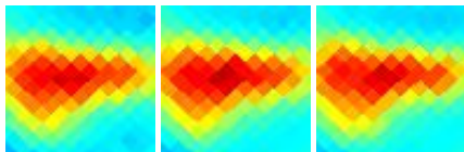
G199.88+00.93 J0630+120
