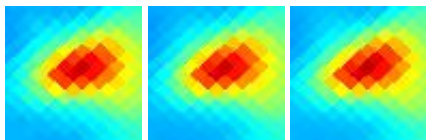
G112.63+20.80 J2058+786
