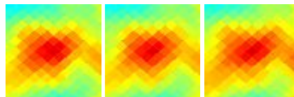
G181.73-19.35 J0440+164
