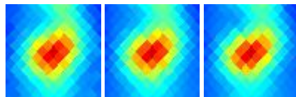
G204.82-13.88 J0547+007
