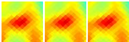
G106.30+13.57 J2122+693
