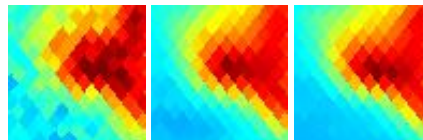
G154.48-15.17 J0330+377
