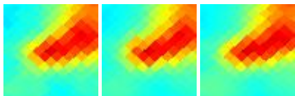
G171.14-17.58 J0418+253
