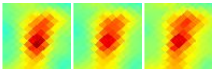
G205.42-08.15 J0608+028
