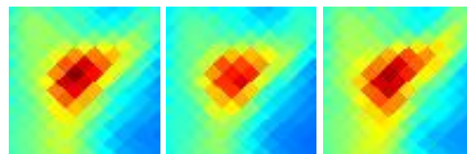
G160.62-16.70 J0348+329
