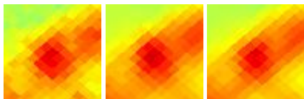
G160.53-19.72 J0338+306
