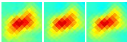
G111.33+19.94 J2057+771
