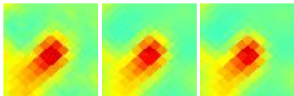
G302.49-16.37 J1242-792
