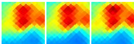
G102.72-25.98 J2324+334
