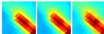
G226.36-00.50 J0714-121
