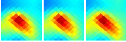
G089.36-00.67 J2112+474
