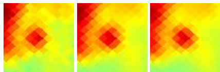
G054.03-02.38 J1940+175
