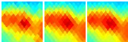
G009.62+21.28 J1652-093
