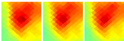
G191.51-00.76 J0608+185
