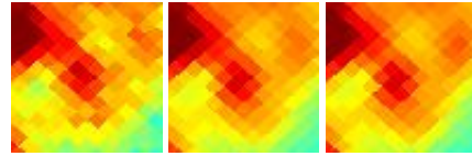
G118.34+08.66 J2355+710
