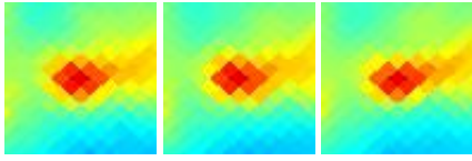
G158.20-20.28 J0329+315
