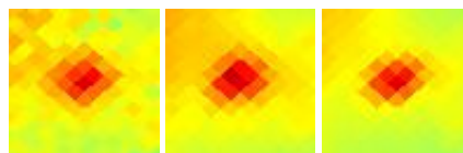
G173.45-13.34 J0439+264
