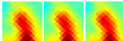
G185.29-02.27 J0549+232
