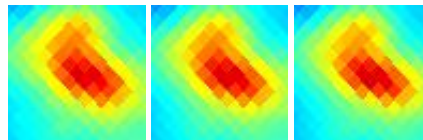
G313.94+02.25 J1417-587
