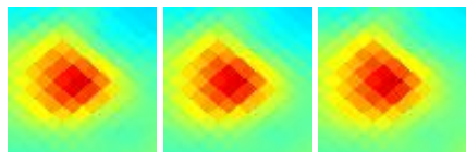
G095.75+08.17 J2056+580
