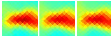
G270.30+02.85 J0925-465
