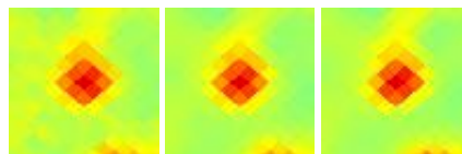
G148.00+00.09 J0354+537
