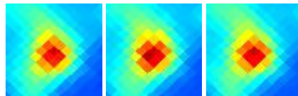
G004.46+16.64 J1656-160
