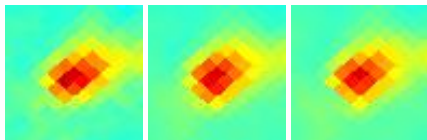
G302.58-15.94 J1244-788
