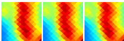
G303.28-13.32 J1257-761
