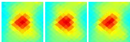
G159.78-24.80 J0322+270
