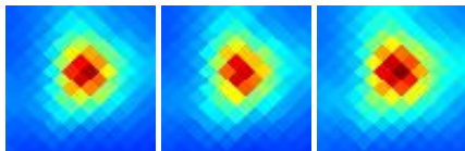
G000.65-00.01 J1747-283
