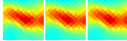
G275.93+01.84 J0946-510
