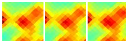
G168.13-16.39 J0413+282
