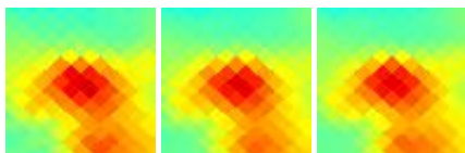
G213.92-13.61 J0604-070
