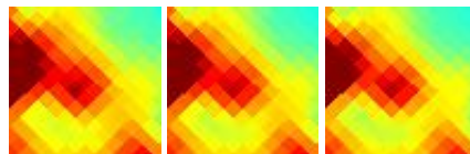
G111.77+20.26 J2057+777
