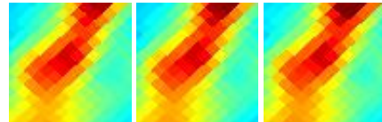
G297.29-16.31 J1103-779
