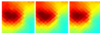
G164.81-05.67 J0440+378
