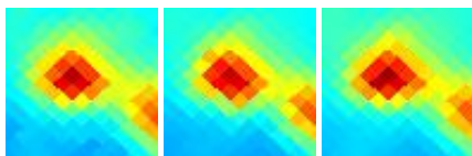
G172.15-09.93 J0447+295
