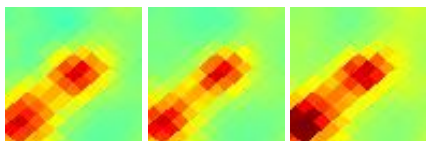
G177.67-20.20 J0427+189
