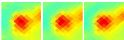
G170.83-15.90 J0423+266
