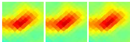
G097.09+10.12 J2051+603
