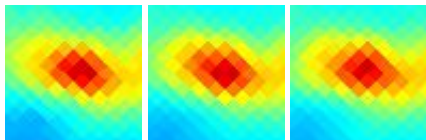
G160.64-35.04 J0258+183
