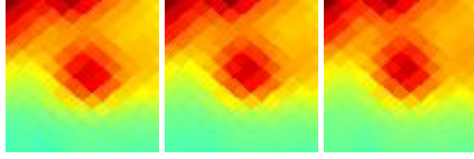
G090.76-04.55 J2134+456
