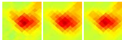
G170.26-16.02 J0421+269
