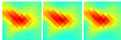
G110.52+19.17 J2100+761
