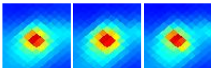
G001.27+03.78 J1734-258
