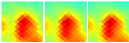
G133.28+08.81 J0251+692
