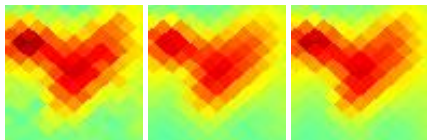
G302.08+07.46 J1245-553
