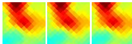
G177.89-20.16 J0428+188
