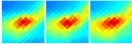
G355.67+14.43 J1641-240
