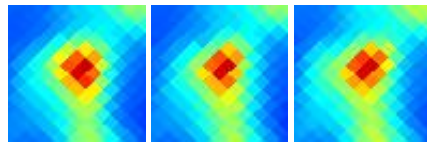
G159.21-20.12 J0333+311
