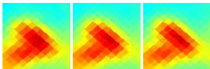
G325.17+05.86 J1517-506
