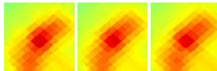
G058.16+03.50 J1926+239
