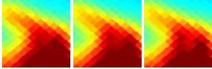
G274.43+00.27 J0932-512
