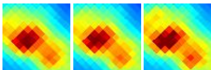
G212.18+05.11 J0708+029
