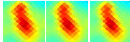
G296.89-14.49 J1110-761
