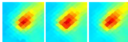
G172.13-16.93 J0423+250
