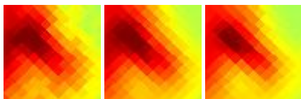
G020.52+01.69 J1822-102
