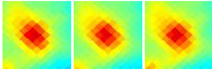
G158.22-20.14 J0329+316
