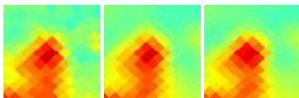
G168.00-15.69 J0415+288
