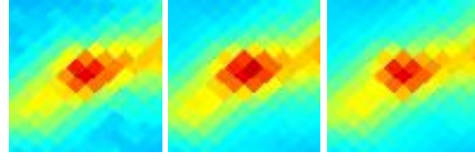
G339.16+15.96 J1545-343
