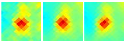
G168.46-17.93 J0409+269
