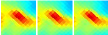
G296.52-01.19 J1153-633
