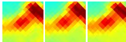
G008.67+22.14 J1647-095
