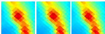
G301.04-15.83 J1214-785
