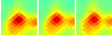
G091.73+04.36 J2058+525
