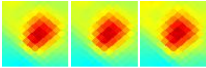
G084.79-01.11 J2056+437
