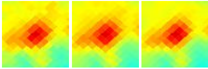
G232.95+00.91 J0732-173
