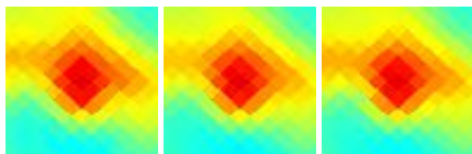
G128.95-00.18 J0143+620
