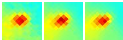
G175.53+01.34 J0539+334
