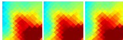
G161.08-21.78 J0334+287
