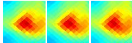
G271.82+04.89 J0939-460
