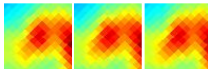
G178.48-06.76 J0516+264
