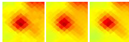
G057.26+04.01 J1922+234
