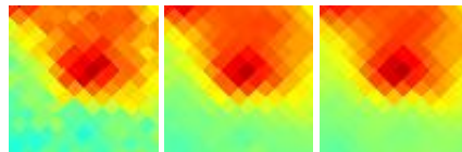
G161.43-35.59 J0259+175
