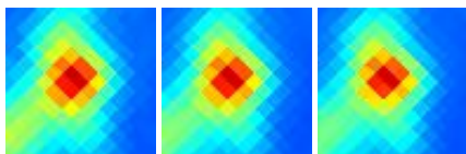
G319.35+00.87 J1459-578
