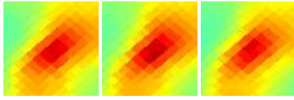
G157.60-12.17 J0351+382
