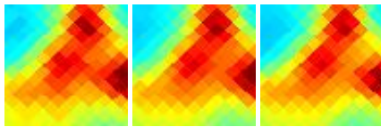
G146.05+17.81 J0536+667
