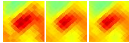
G125.70+12.52 J0133+751
