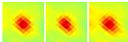
G023.33+11.81 J1751-029
