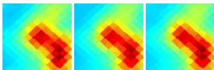
G300.21-03.47 J1224-662
