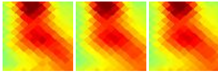
G144.66+06.11 J0405+605
