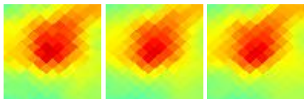
G203.75-08.49 J0604+041
