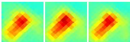
G175.20+01.28 J0538+336
