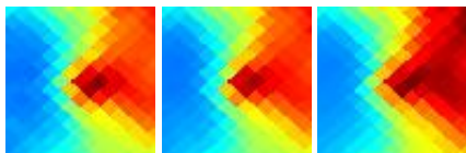
G194.69-16.84 J0517+077
