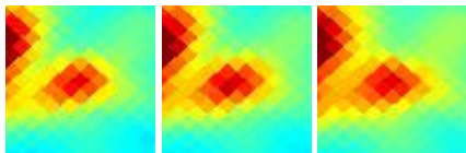
G336.90-03.09 J1649-496
