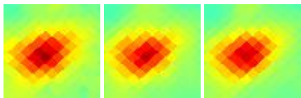
G170.88-10.92 J0440+299
