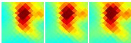
G216.18-15.24 J0602-097
