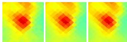
G300.80-09.08 J1224-718
