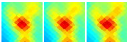
G220.95-08.32 J0636-108
