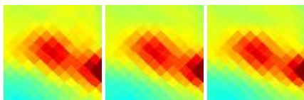
G111.42+19.82 J2100+771
