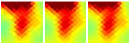
G132.29+09.36 J0244+701
