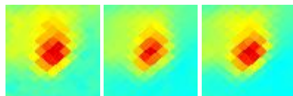
G203.57-30.08 J0447-059
