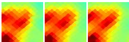
G202.58-08.70 J0601+051
