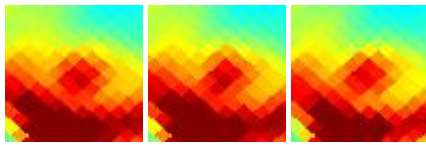
G159.21-20.44 J0332+308
