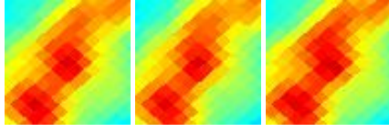
G157.25-01.00 J0432+466
