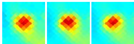
G172.33-18.24 J0420+240
