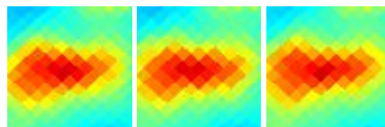
G174.22-13.43 J0441+258
