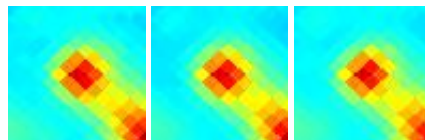
G128.25+20.78 J0325+820
