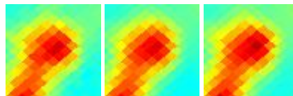
G048.82-03.82 J1934+122
