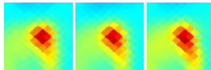
G061.76-10.80 J2027+196
