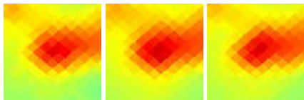
G209.20+02.12 J0652+042
