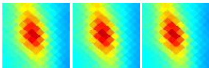
G300.87-08.95 J1225-717
