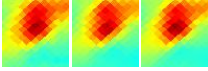
G157.19-08.81 J0401+410
