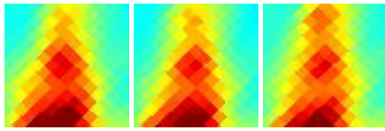
G158.40-21.86 J0325+301
