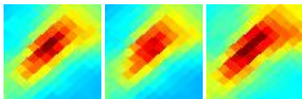
G165.34-07.51 J0435+362
