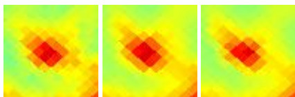
G300.62-09.61 J1221-723
