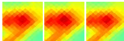
G179.14-06.27 J0519+262
