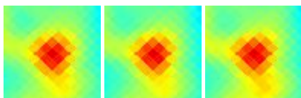
G114.16+14.80 J2230+752
