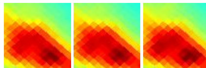
G150.44+03.95 J0425+549
