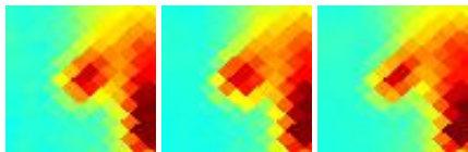
G171.78-15.65 J0426+261
