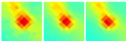
G021.26+12.12 J1746-045
