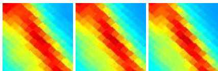
G301.39-07.97 J1232-707
