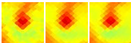
G149.23+03.07 J0414+552
