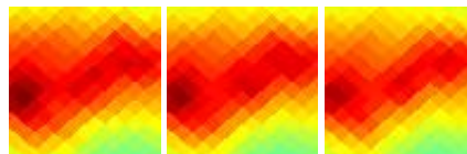
G164.94-05.71 J0441+377
