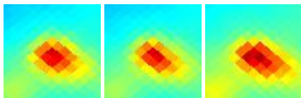
G023.68+07.53 J1807-046
