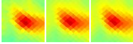
G092.02+03.93 J2102+524
