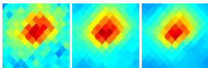
G174.08-13.24 J0441+260
