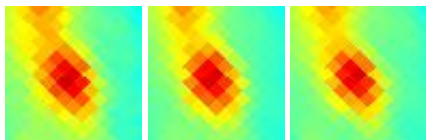
G006.32+20.44 J1647-123
