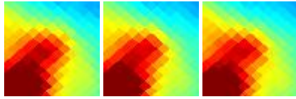
G357.97+13.15 J1652-231
