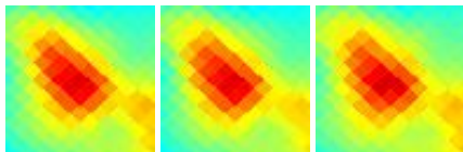
G207.35-19.82 J0530-042
