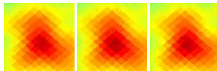
G129.94+11.73 J0229+732
