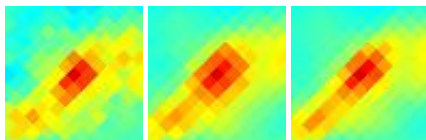
G164.94-08.57 J0430+358
