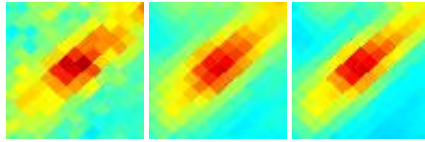
G236.68-05.21 J0717-234
