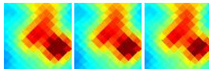
G112.03+17.89 J2132+763
