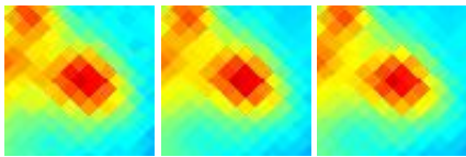
G145.87+17.77 J0535+668
