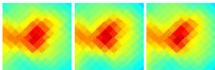
G175.34-10.82 J0453+265
