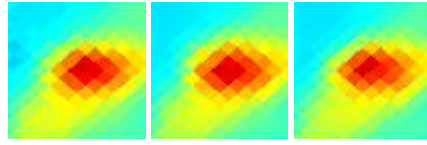
G157.91-08.23 J0406+410
