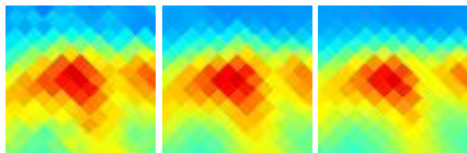
G028.45-06.39 J1906-068
