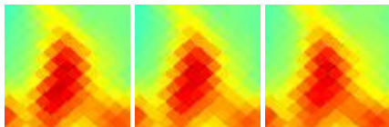
G028.56-00.24 J1844-039
