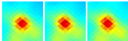
G058.02+03.02 J1928+236
