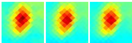
G180.81-19.66 J0437+169
