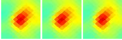
G290.96-03.48 J1059-637
