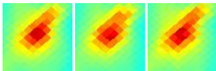
G178.98-06.74 J0517+260
