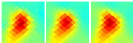
G336.64+08.23 J1601-418
