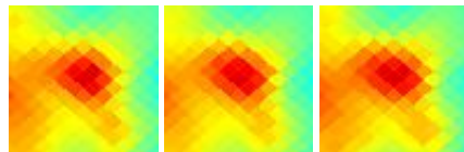
G210.01-20.16 J0534-065
