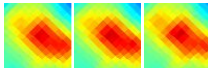
G160.33+03.24 J0502+470
