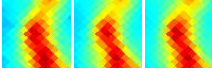
G339.14+16.10 J1545-342
