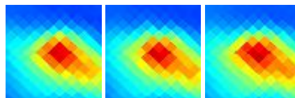
G172.30-09.91 J0448+294
