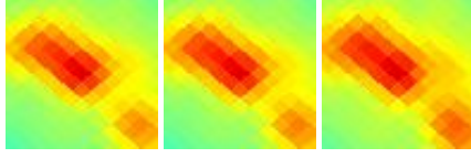
G089.75-02.16 J2120+466
