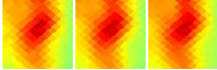
G296.21-15.83 J1050-770
