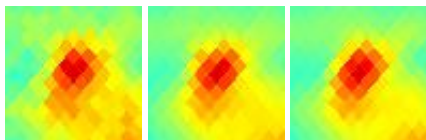
G159.67-05.71 J0422+416
