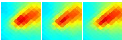
G179.29+04.20 J0600+316
