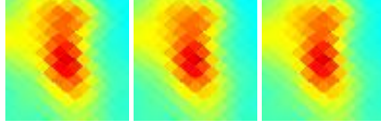
G247.65+00.29 J0802-303
