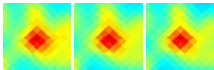
G102.17+07.27 J2137+620
