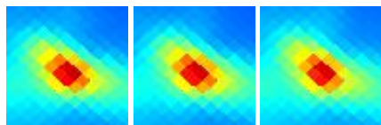
G095.11+06.50 J2103+564
