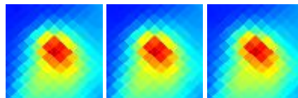
G303.72-14.86 J1305-777
