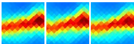
G169.84-07.61 J0449+328
