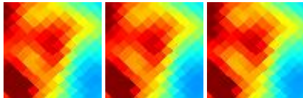
G297.22-15.63 J1107-773
