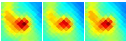
G170.13-16.06 J0420+270
