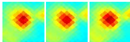
G206.60-14.40 J0548-010
