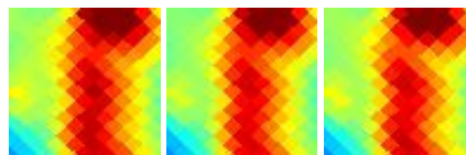
G303.39-14.26 J1259-771
