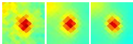
G043.02+08.36 J1839+127
