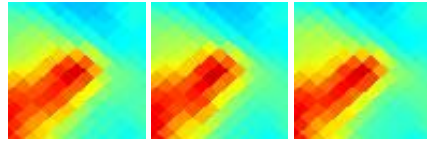
G157.12-11.56 J0351+390
