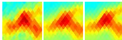
G153.74+35.91 J0836+624
