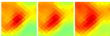
G001.64-00.07 J1749-275
