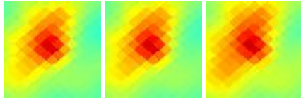
G089.03-41.28 J2308+147
