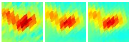
G167.23-15.32 J0414+295
